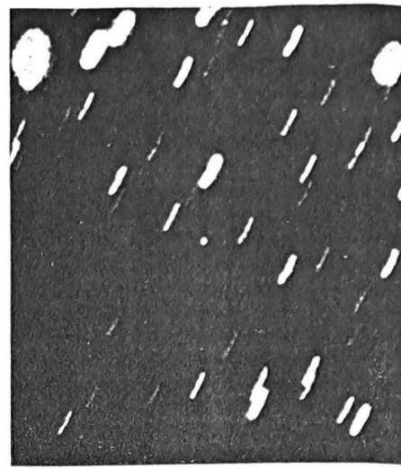
Three examples from astronomical photography illustrate some of the principles of observing the satellite. At the left is a Harvard photograph of a Geminid meteor whose trail has breaks caused by a rotating shutter in the camera; the meteor's motion can be measured from these breaks. In the center, the trail of an asteroid is recorded on a long-exposure photograph guided on the stars, but for a fainter object, as in the third picture, it is better to shift the camera to follow the moving asteroid, which then appears as a bright point while the star images are trailed. Photographs from Harvard Observatory and Goethe Link Observatory.
