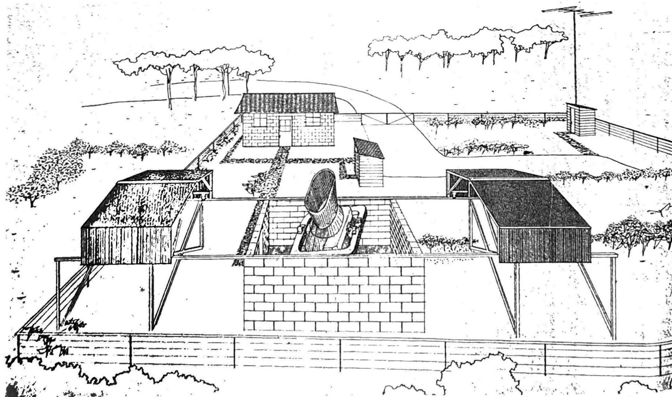
An artist's conception of the layout for a typical satellite-tracking camera station. In the foreground, the camera is seen in observing position. The roof of the camera shelter, which measures 14 by 14 feet, divides into two parts. These slide far apart so there is no obstruction to quick pointing of the camera in any direction. In the background is the combined office-shop and a power shack; in the upper right is the radio antenna, just behind a small fuel-storage building. Smithsonian Astrophysical Observatory drawing by Naibu Akashi.
