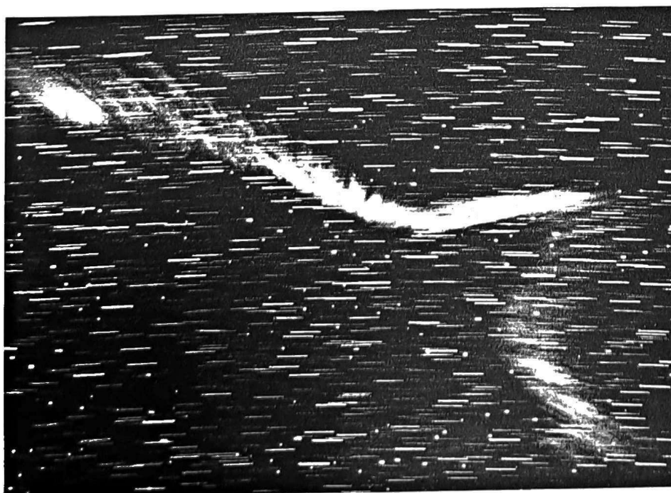
Fig. 7. The Schmidt camera was used without drive for this one-minute exposure of the train of the same fireball, 2½ minutes after the meteor disappeared. The inconspicuous kink of Fig. 6 is now very noticeable at the right.
