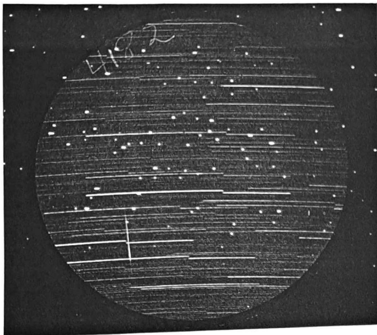
Fig. 3. A contact print of a typical three-minute search exposure with the Schmidt camera, on April 19, 1955. The driving rate of the camera was 190 degrees per hour. Note the declination offset, which divides each star trail into two parts. During the exposure, a bright meteor crossed the field (lower left); thickenings of its trail indicate bursts of light.
