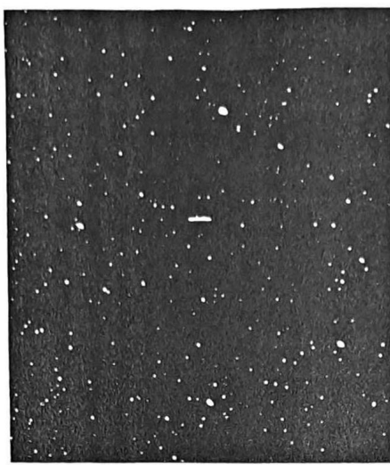
Three examples from astronomical photography illustrate some of the principles of observing the satellite. At the left is a Harvard photograph of a Geminid meteor whose trail has breaks caused by a rotating shutter in the camera; the meteor's motion can be measured from these breaks. In the center, the trail of an asteroid is recorded on a long-exposure photograph guided on the stars, but for a fainter object, as in the third picture, it is better to shift the camera to follow the moving asteroid, which then appears as a bright point while the star images are trailed. Photographs from Harvard Observatory and Goethe Link Observatory.
