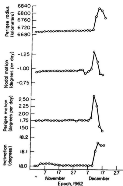
FIG. 7. Behavior of some Explorer 15 orbital parameters in late 1962.
