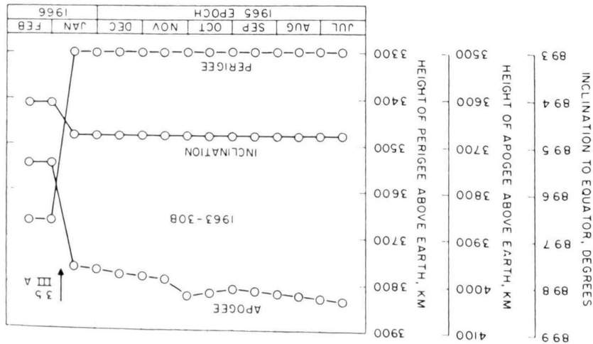
FIG. 4. Orbital parameters of Satellite 1963-30B during late 1965 and early 1966.
