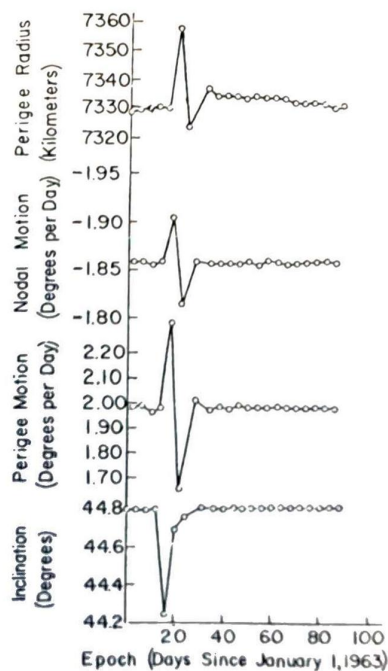
FIG. 1. Behavior of some Telstar 1 orbital parameters in early 1963.
