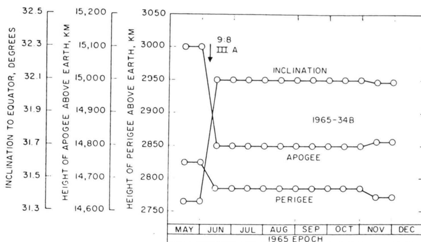
FIG. 6. Orbital parameters of Satellite 1965-34B during 1965.
