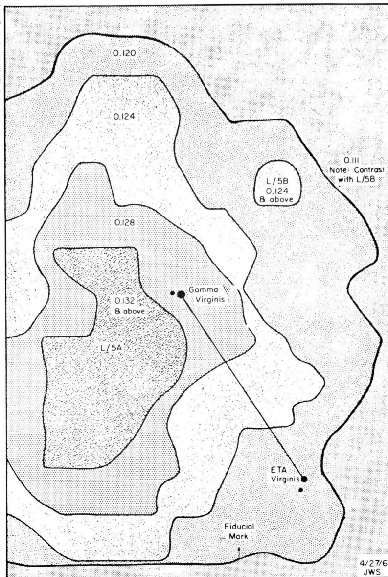
DENSITY-GRADIENT contour plot of the L/5 lunar libration-cloud photograph taken from the ground 13 Feb. 1966. The number in each shaded band is the ratio of the differential image density to background density. The vertical and horizontal scales are different and the angular area of the diagram is 10 deg by 10 deg. —FIG. 3
