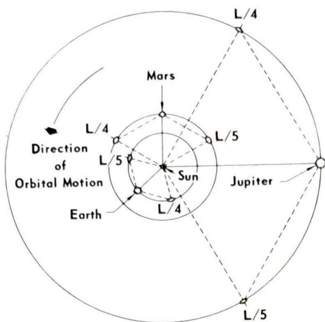
SEXTILE libration points of three sun-planet systems. —FIG. 1
