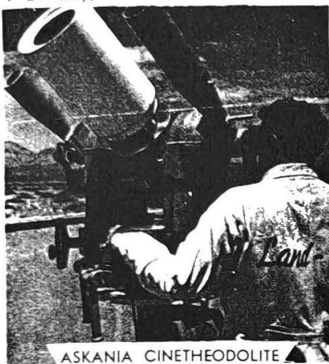
ASKANIA CINETHEODOLITE
