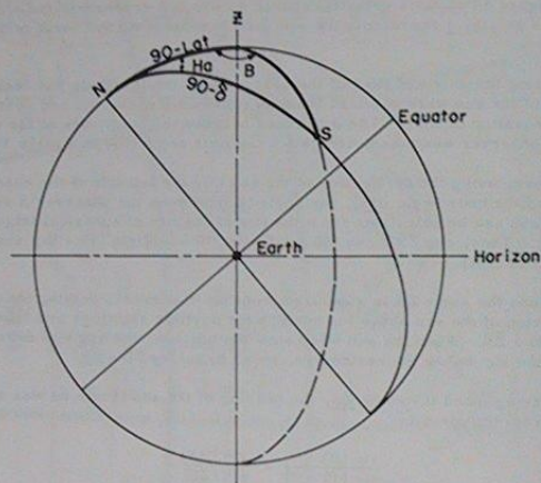
FIGURE 39 DIAGRAM OF A CELESTIAL SPHERE
