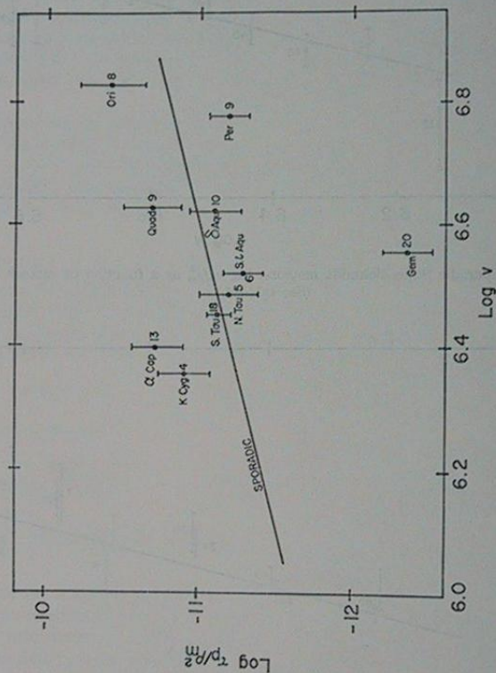
FIGURE 4.—Super-Schmidt shower meteors: mean values and standard deviations of \log \tau_e/\rho_e^2 for the principal showers. (See table 5.)
