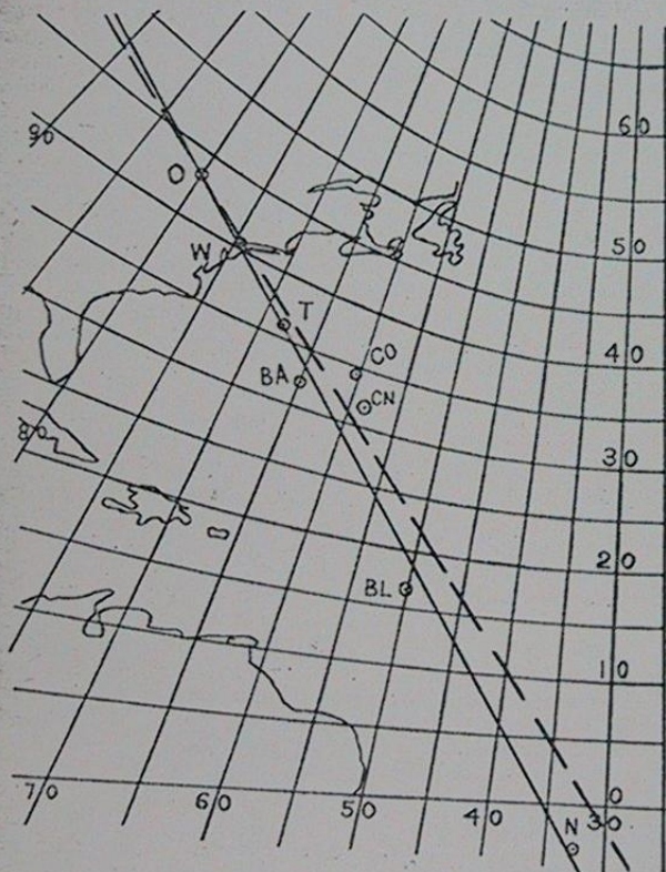
GREAT CIRCLE CHART OF OBSERVERS' STATIONS, 1913 FEBRUARY 9.
