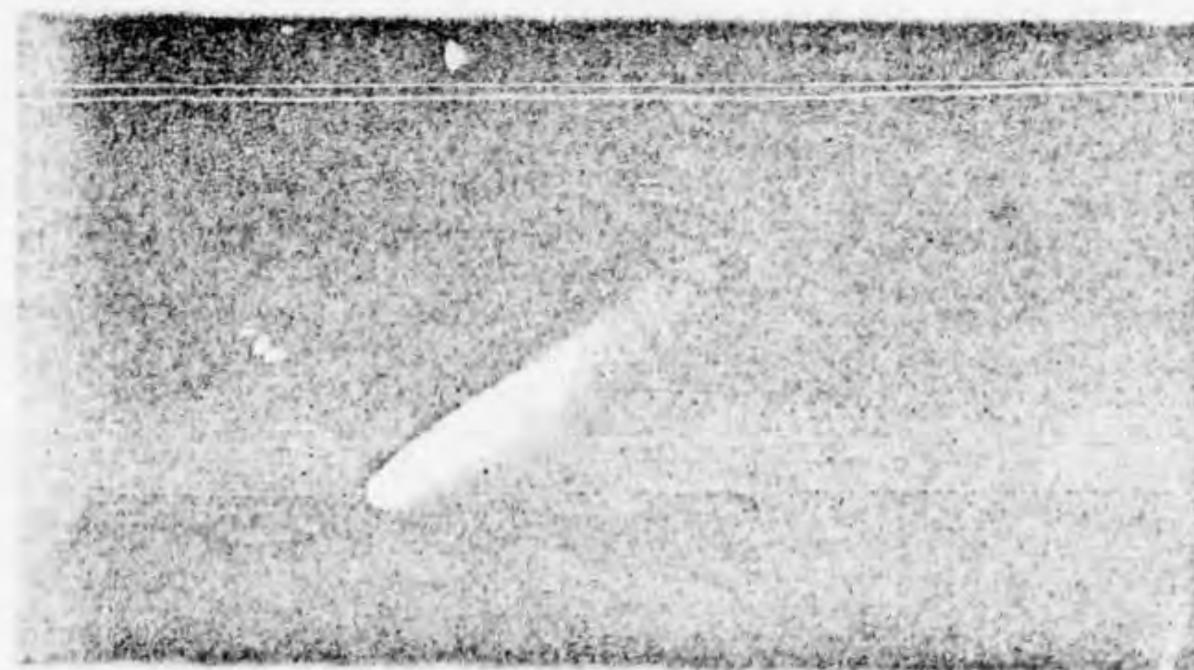
NEW COMET and its tail appear as a ball of light in this photograph made with the 14-inch telescope camera at Palomar mountain observatory. Most of comet's glow is light which is scattered from the sun and then reflected.
