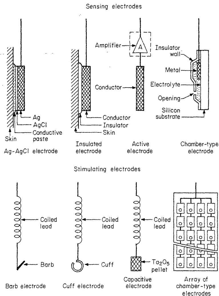
Fig. 26-46. Types of electrodes.
