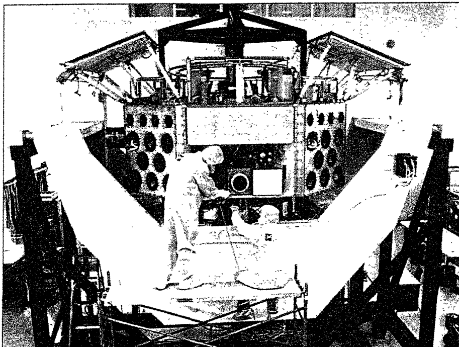
Engineers check cradled CRRES satellite in Ball Aerospace's clean room
