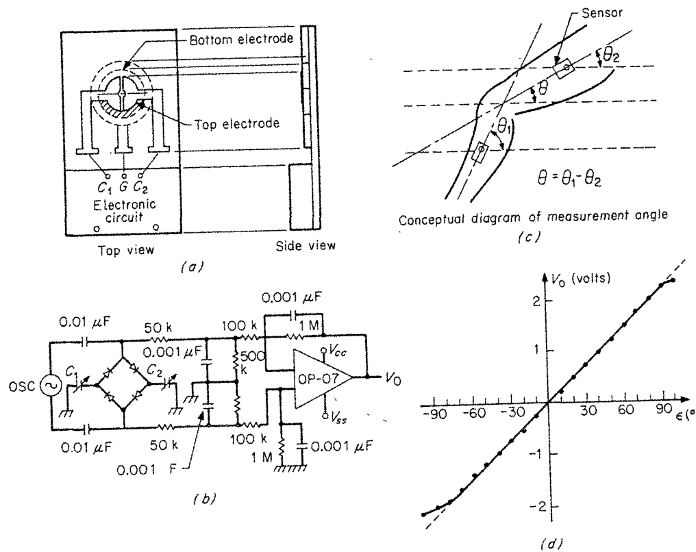
Fig. 26-48. The principle and structure of a joint angle sensor: (a) structure, (b) circuit, (c) principle, (d) results.
