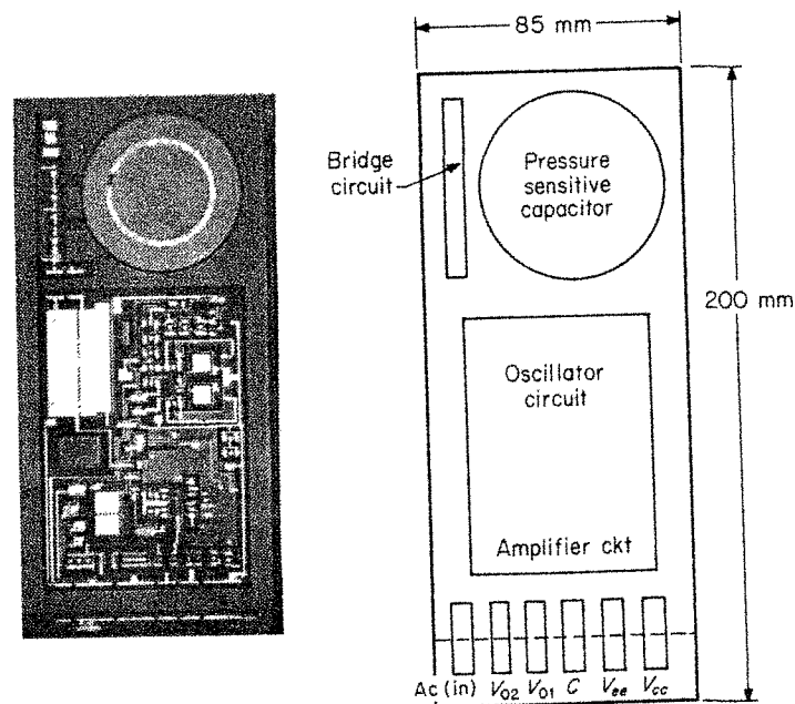
Fig. 26-49. A silicon capacitive pressure transducer with a bipolar signal-processing circuit on the chip.
