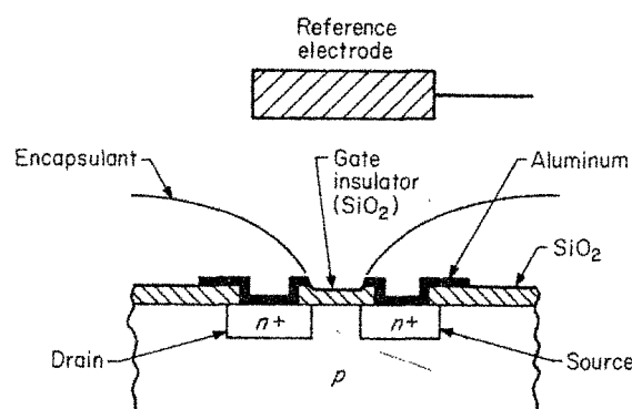
Fig. 26-50. Structure of silicon-dioxide-gate ISFET.
