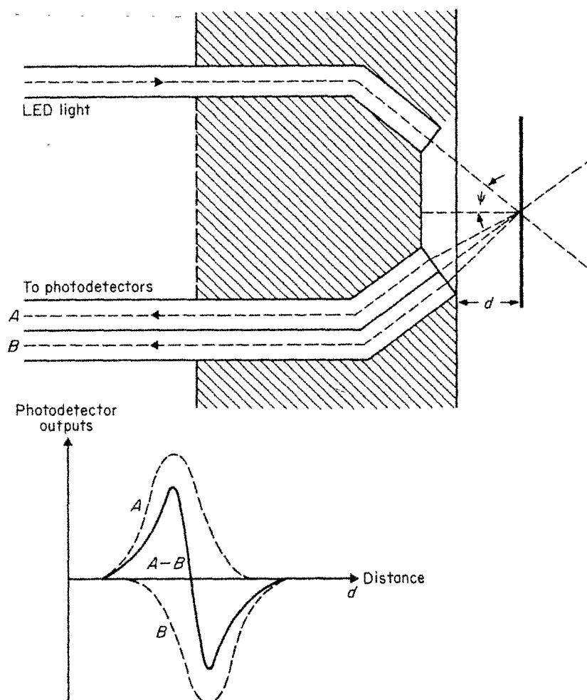
Fig. 26-47. Principle of optical position detector.
