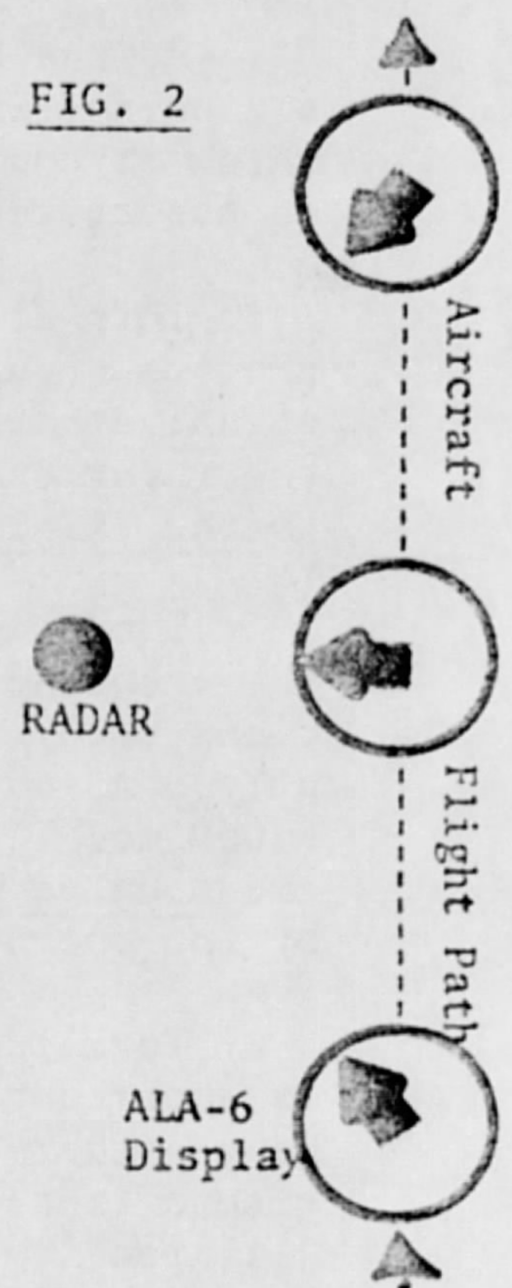
NORMAL OPERATION of AN/ALA-6 Elint Direction-Finder
