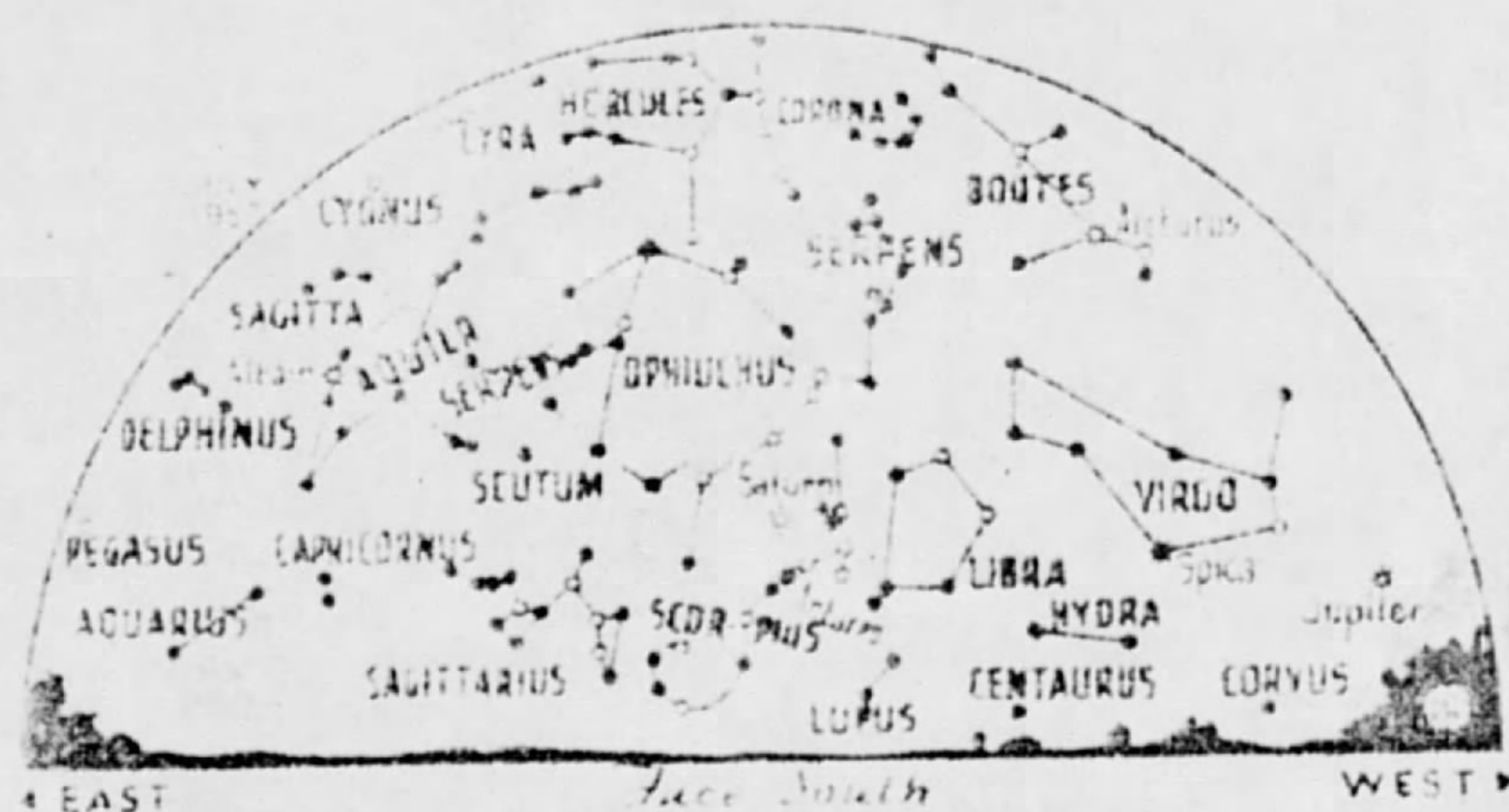
• • • • SYMBOLS FOR STARS IN ORDER OF BRIGHTNESS
