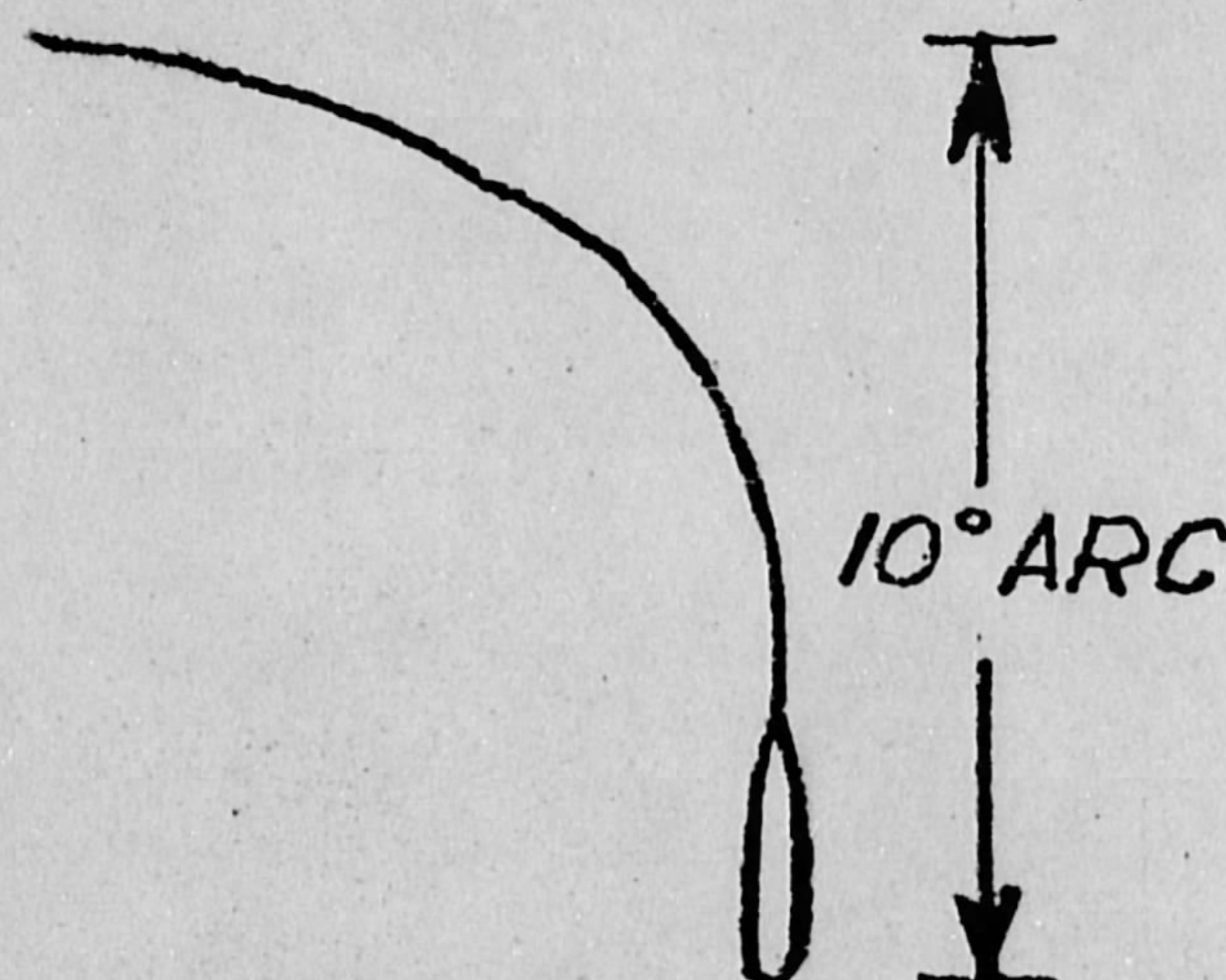
Figure 2. Arc described by light's descent.
