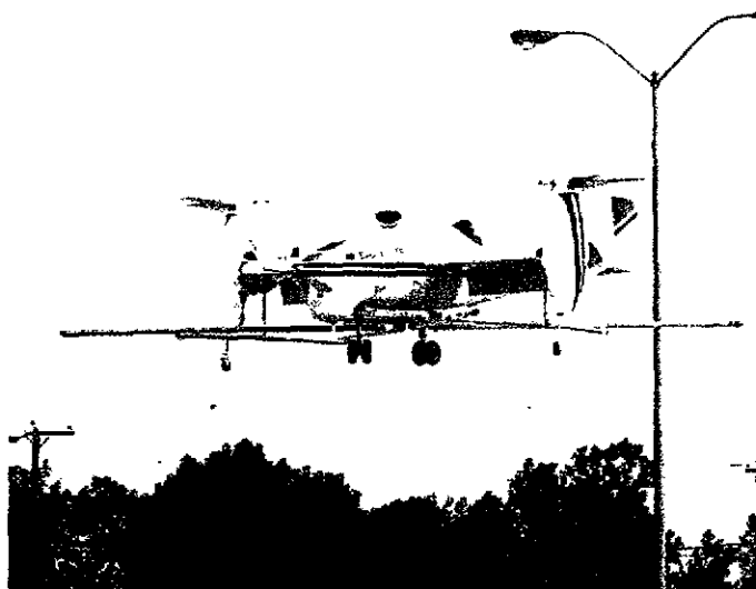
The Bell Eagle Eye tilt-rotor unmanned aerial vehicle made its first flight July 10 in Fort Worth, Texas, but was damaged a few days later in a hard landing on its sixth flight.
