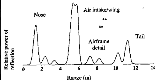
A typical aircraft radar return: each type has its own distinctive features
