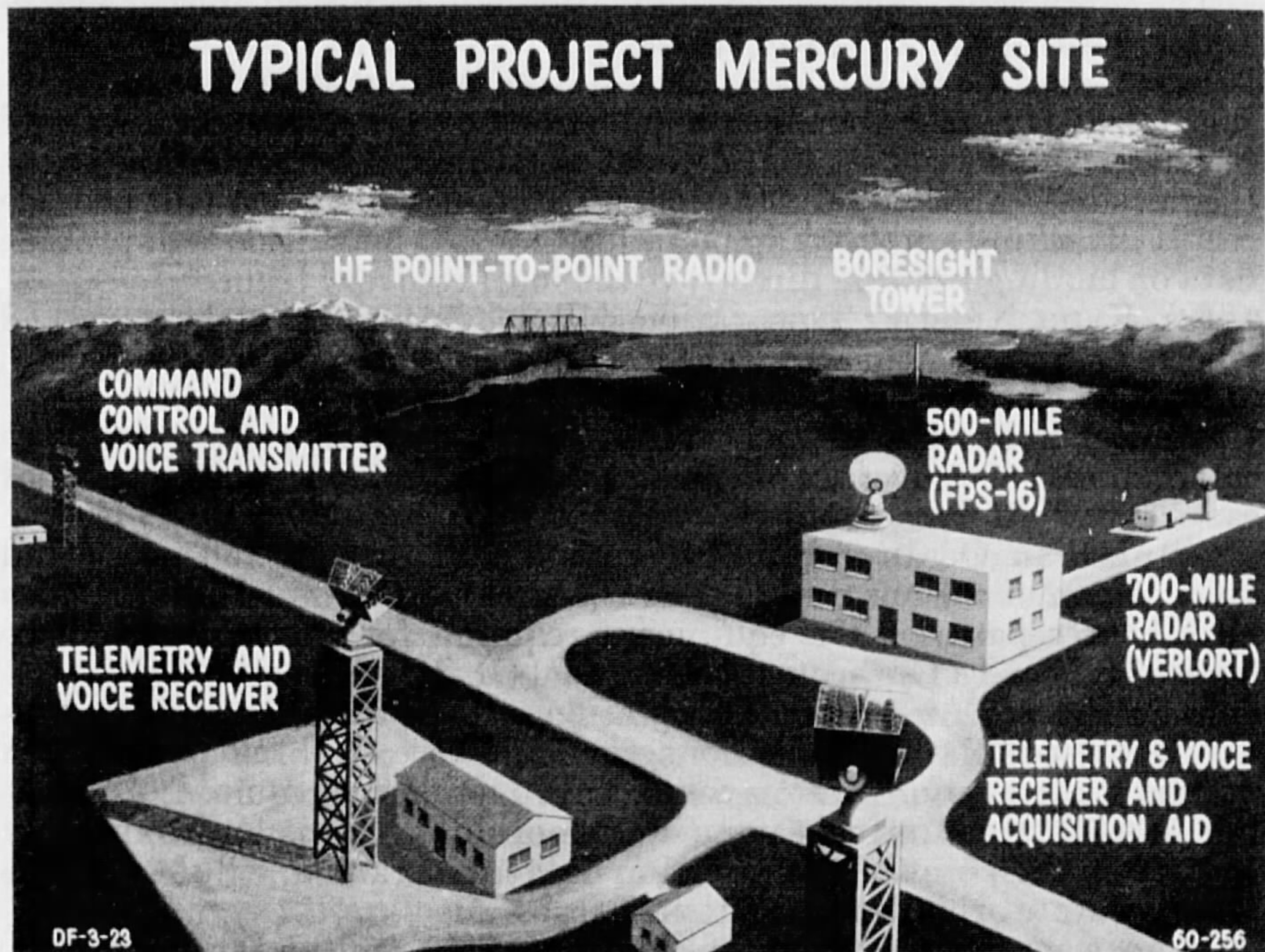
FIGURE 17.—Typical Project Mercury network station.
