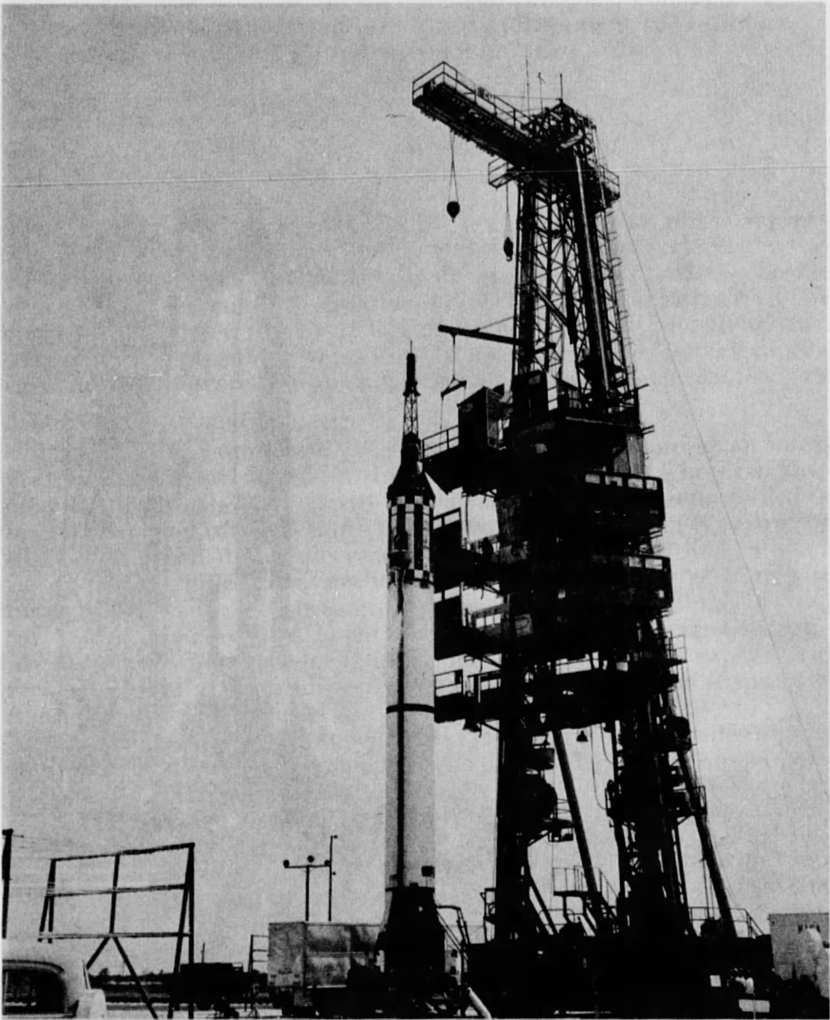
FIGURE 13.—Mercury-Redstone.
