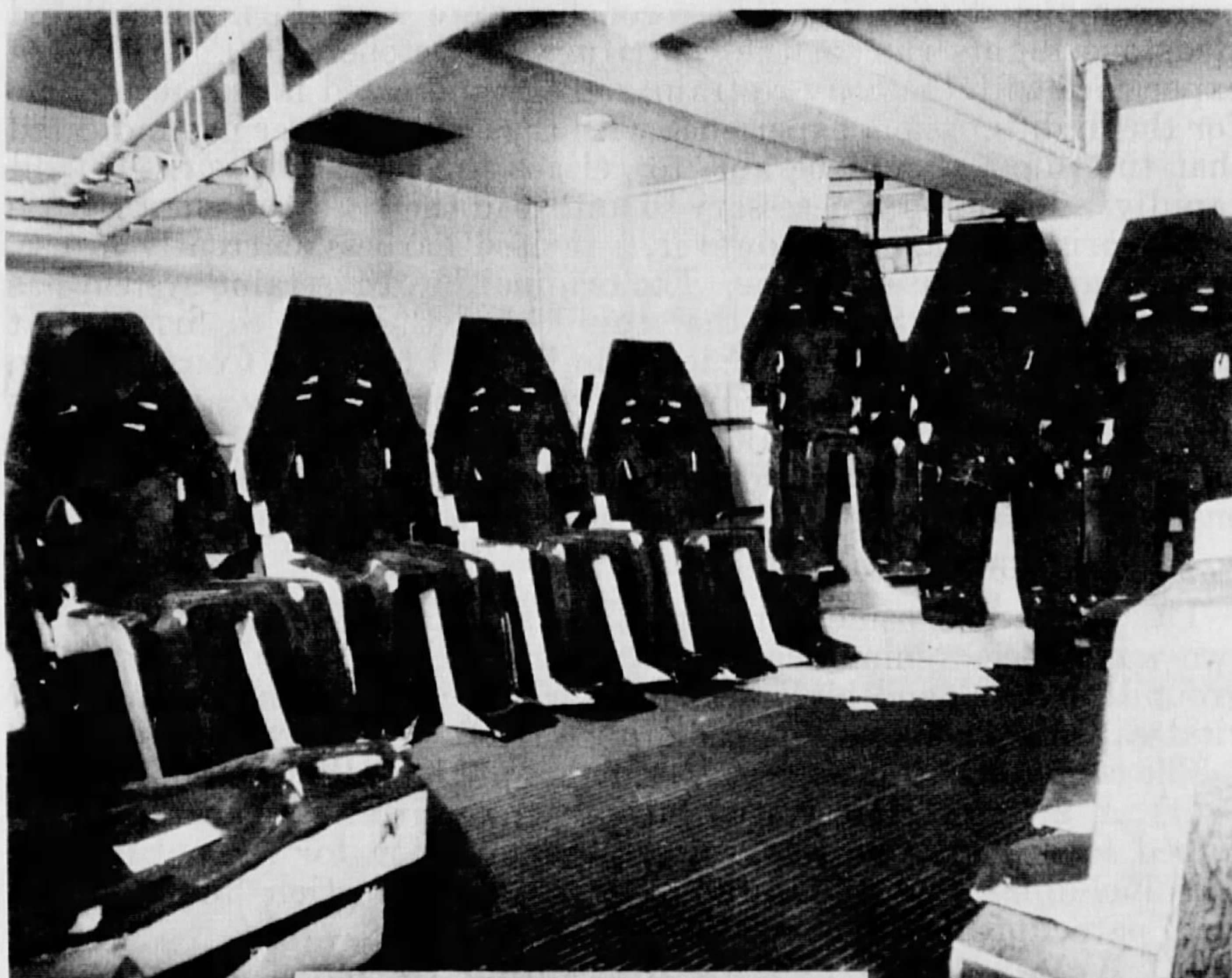
FIGURE 7.—Project Mercury molded couches.
