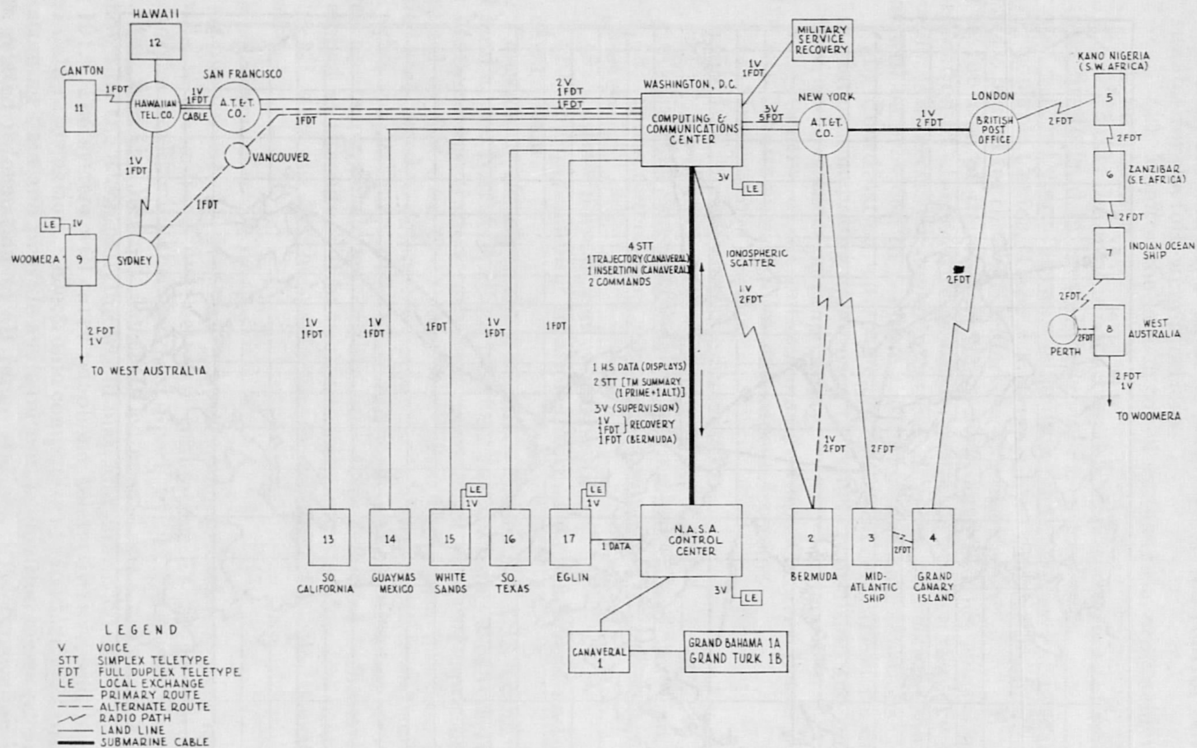
FIGURE 19.—Ground communications circuit layout.
