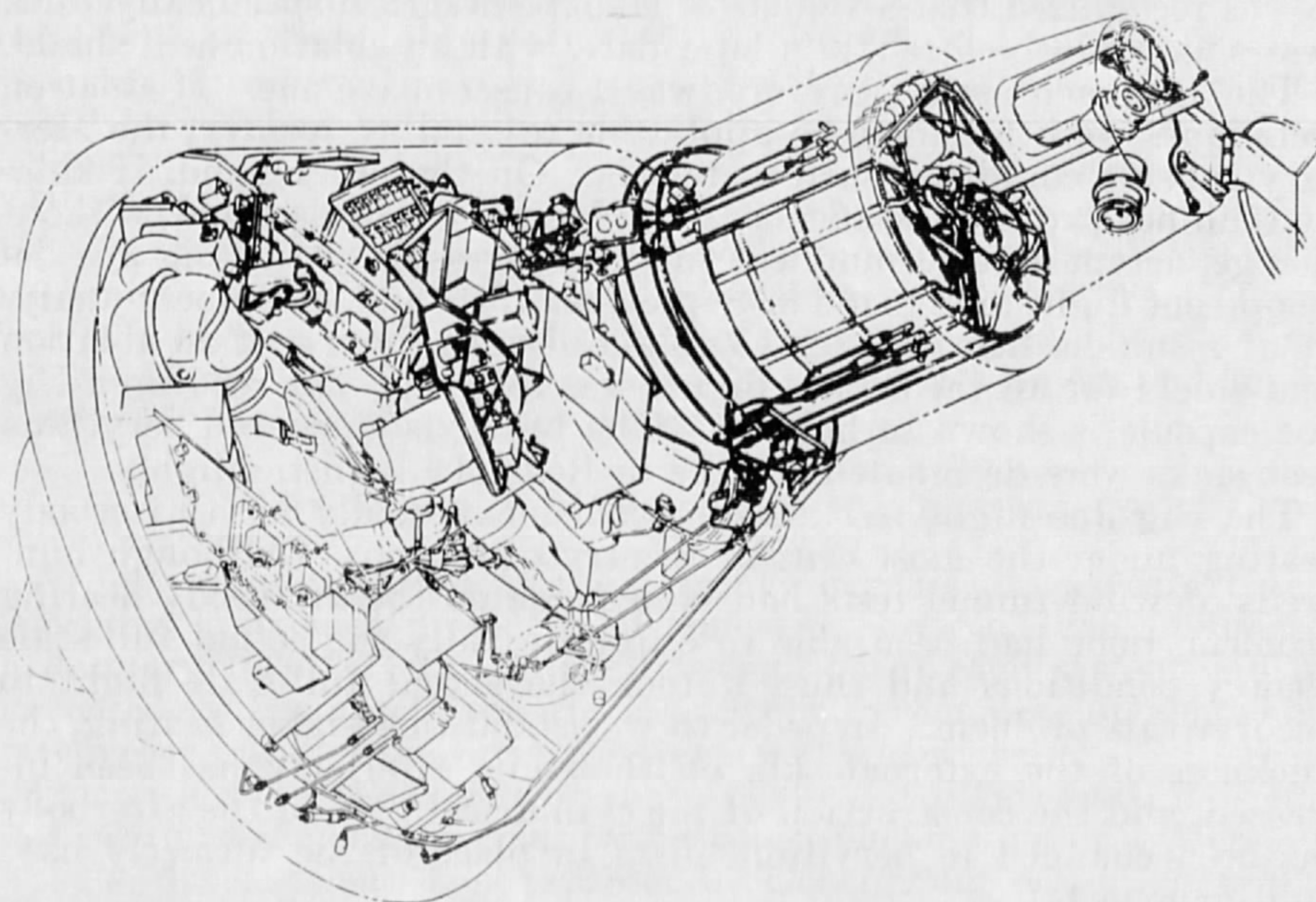
FIGURE 3.—Mercury capsule internal arrangement.
