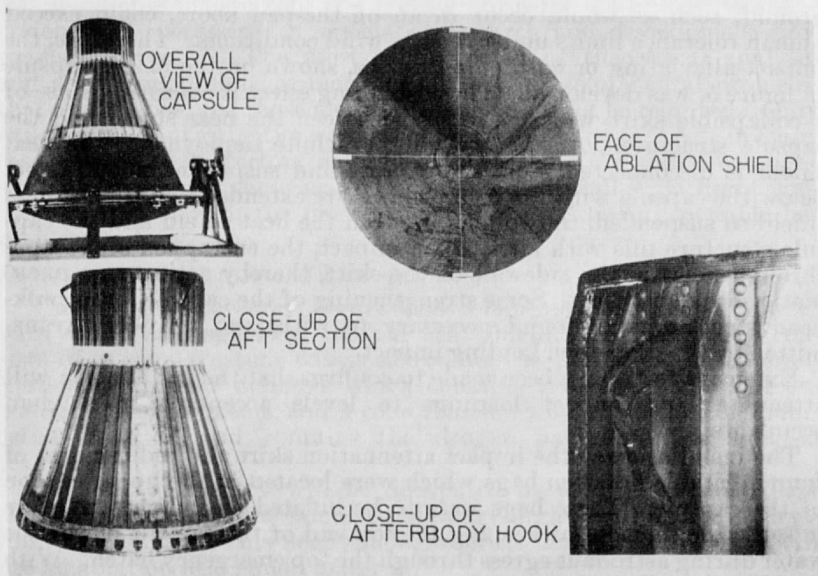
FIGURE 4.—Detailed photographs of recovered Big Joe capsule.
