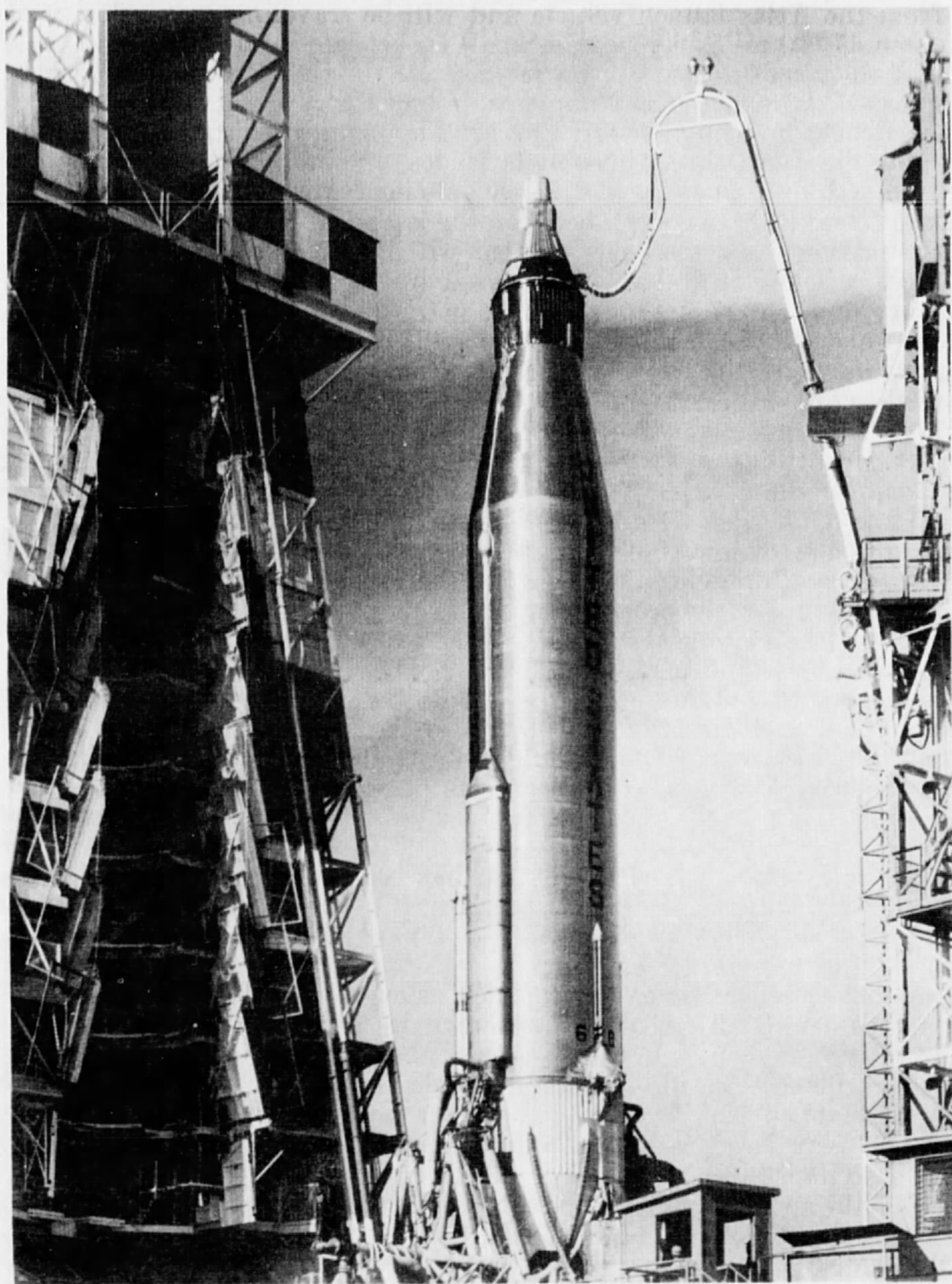
FIGURE 1.—Atlas launch vehicle with development capsule.
