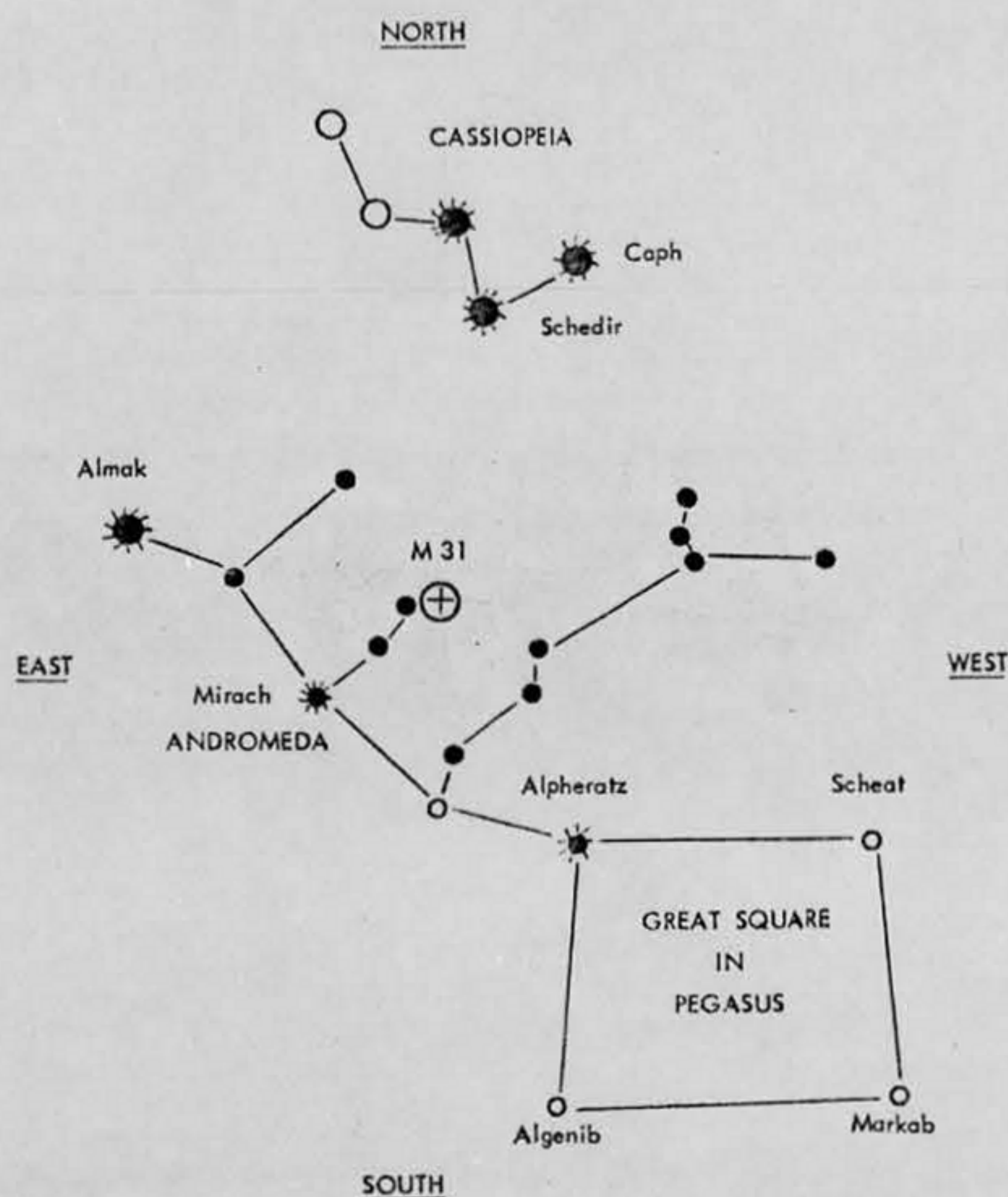
Fig. 1 MAP SHOWING LOCATION OF ANDROMEDA GALAXY -- M 31
