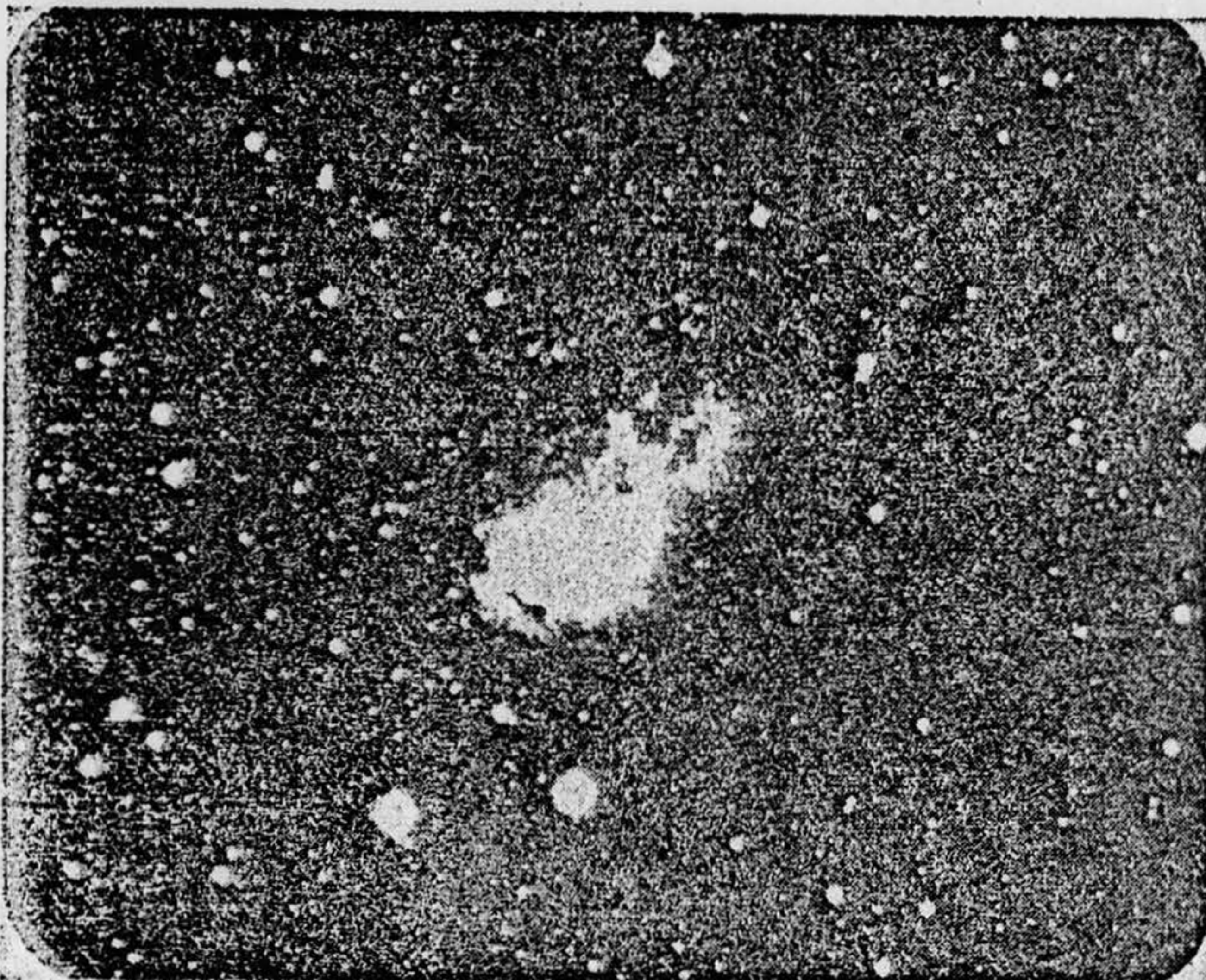
THIS IS PHOTO TAKEN OF GALAXY IC 10 FROM HALE OBSERVATORY It Is Possible Life May Exist In Galaxies Beyond Our Own—UPI
