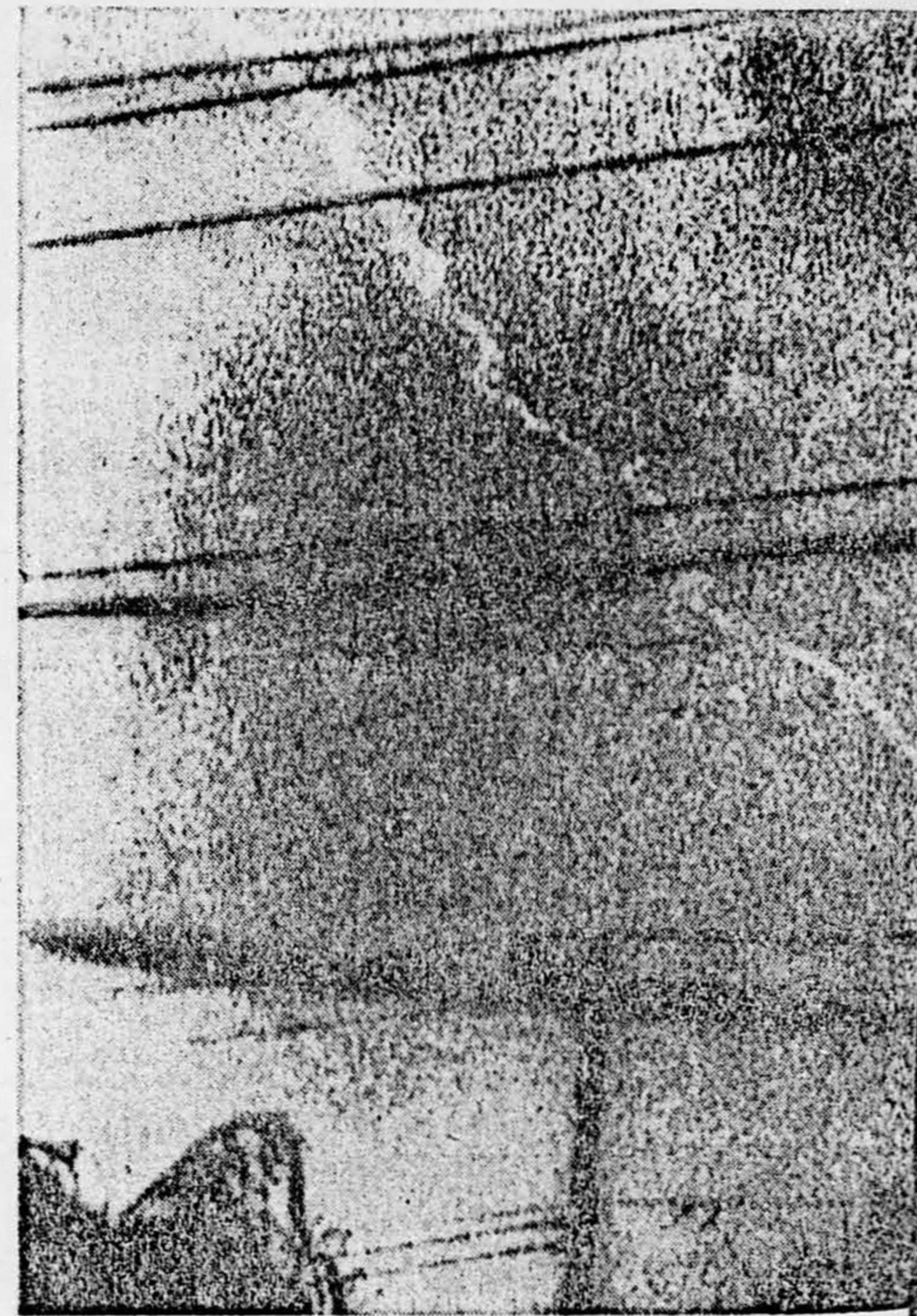
Contrail of Flaming Meteor That Raced Over Northeast
