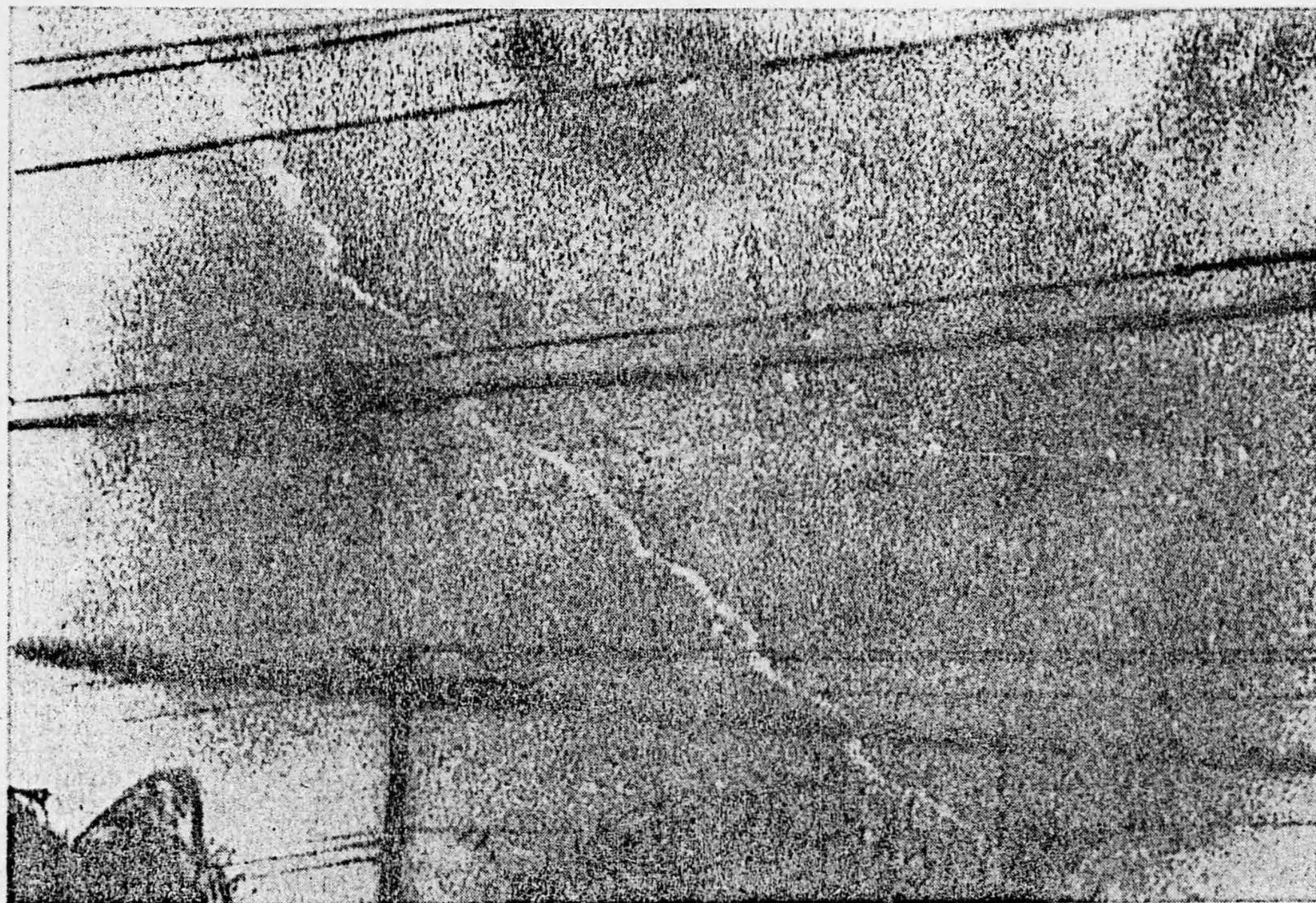
Contrail of Flaming Meteor That Raced Over Northeastern United States; Halo Upper Part of Picture Is Watermark
