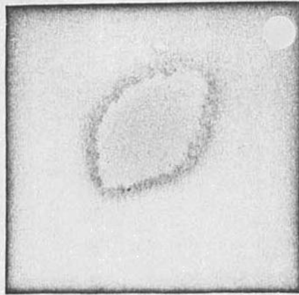
Ionized plasmas produced by electric discharge in laboratories of Illinois Institute of Technology's Research Institute several years ago show some of the characteristic shapes of UFO sightings. However, these pictures were made with extremely short film exposure times of 0.2-0.5 microsec., far briefer than the Lucci photo (below).
