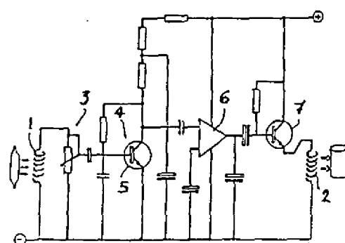
Amplifier Circuit Diagram. 1, input electromagnetic coil; 2, output electromagnetic coil; 3, high frequency filter; 4, preamplifier; 5, transistor; 6, amplifier; 7, common transistor.
