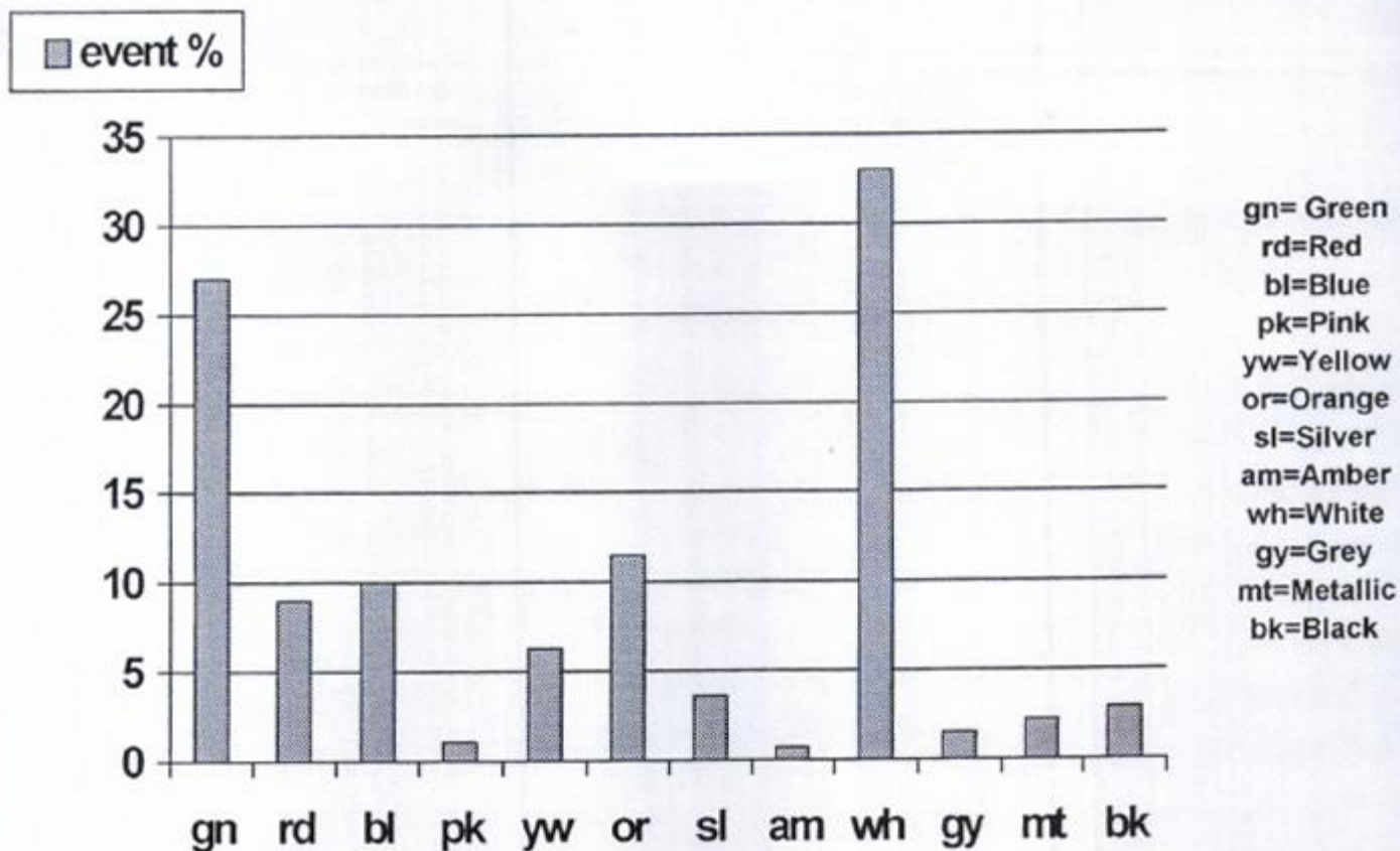
FIGURE 3-6 ANALYSIS OF UAP COLOURS(U)
