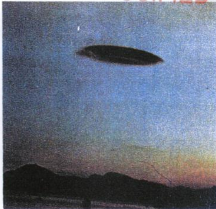
FIGURE 3: LENTICULAR CLOUD
