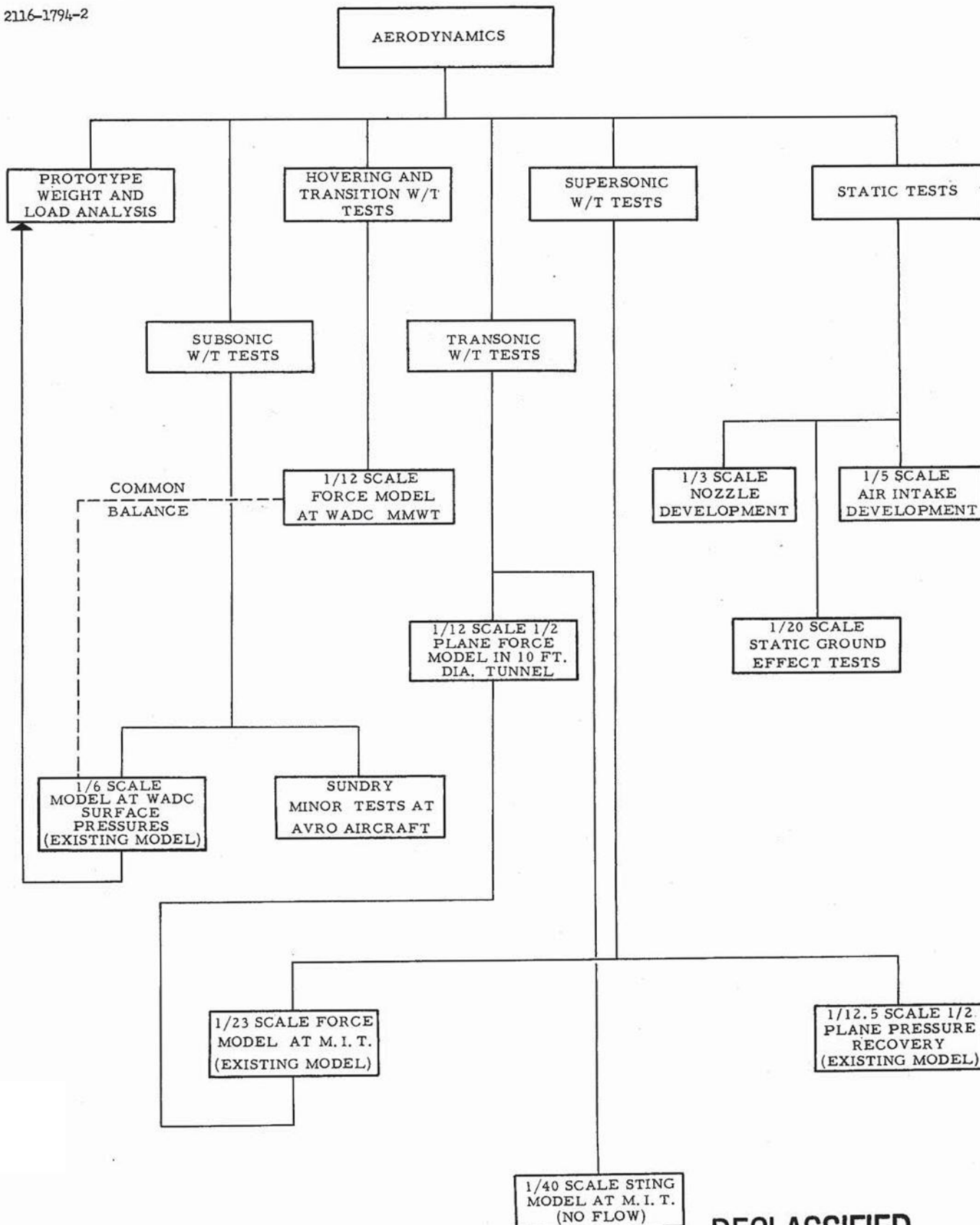
FIG. 30 WORK CHART - AERODYNAMICS
