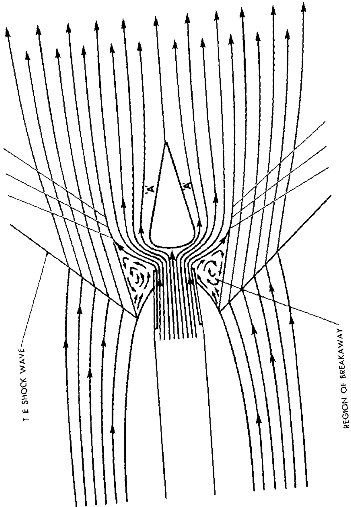
Fig. 9 Section Through Rear of Aircraft at Supersonic Spe
