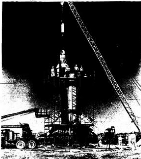
FIGURE 8.—Little Joe launch vehicle during capsule mating operations.
